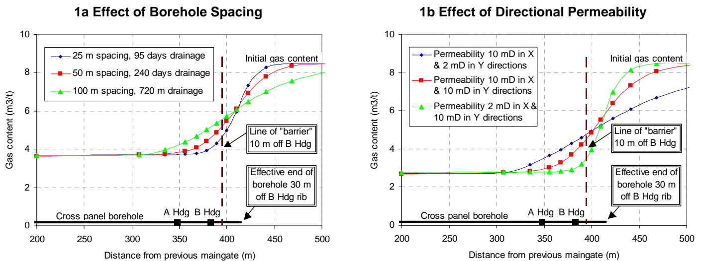
Figure 1 Increase in Remaining Gas Content Approaching the End of a Borehole
