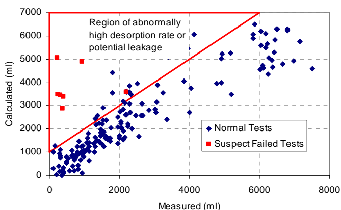
Figure 5 Identifying Abnormal Data Based on “Q2 Initial”
