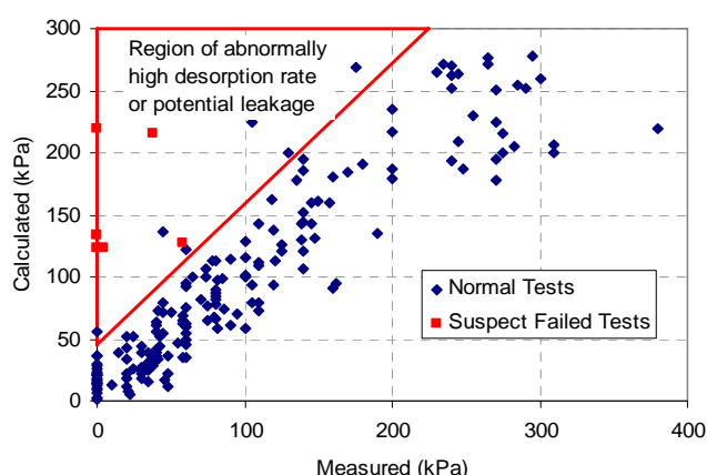
Figure 6 Identifying Abnormal Data Based on Canister Pressure
