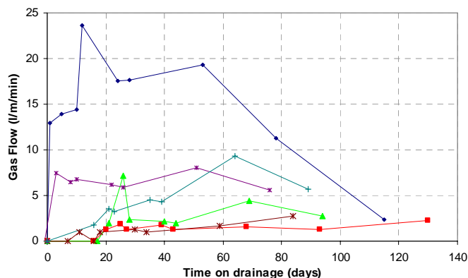
Figure 3b Variable Gas Drainage
