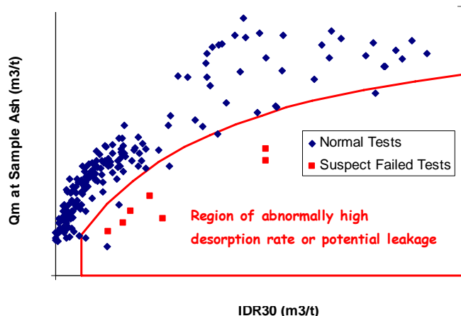
Figure 4 Identifying Abnormal Data Based on Initial Desorption Rate
