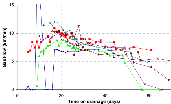
Figure 3a Uniform Gas Drainage
