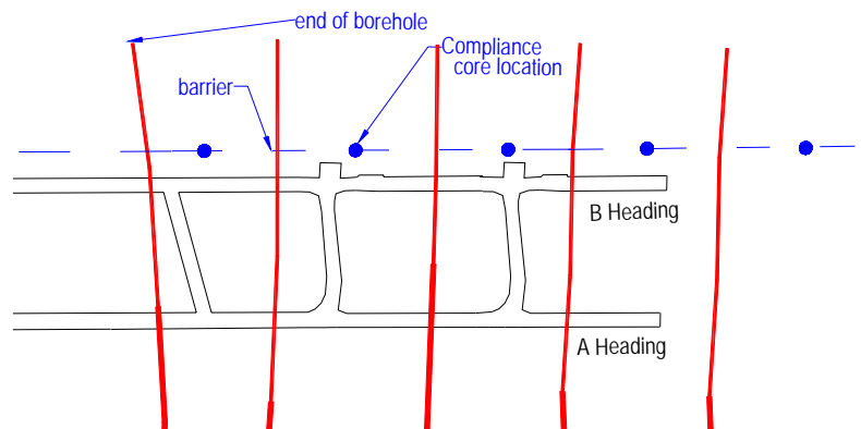
Figure 2 Compliance Core Locations
