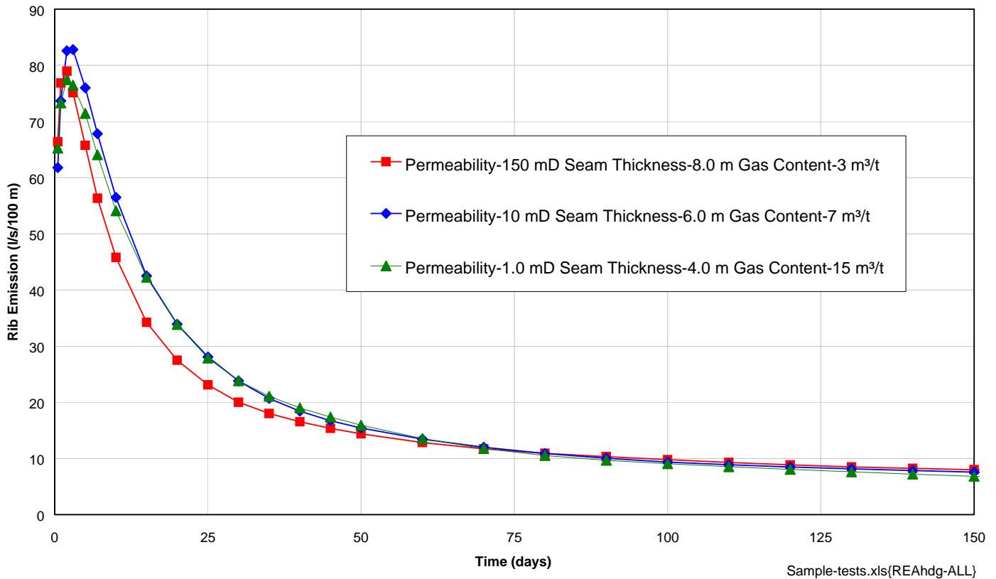
Fig. 3 – Rib Emission Decay Curves Showing Compensating Effects Between Gas Content, Permeability and Seam Thickness
