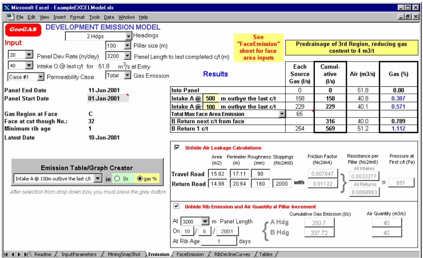
Figure 5 Example of Interactive Worksheet “EXCEL” Model
